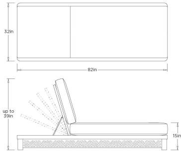
FTS04 EMOTO OUTDOOR CHAISE ARTERIO RS
