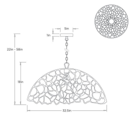
*ADDITIONAL CHAIN AVAILABLE DMI35 LOTUS PENDANT ARTERIO RS
